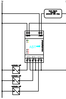
ASTmidi 3 outputs
